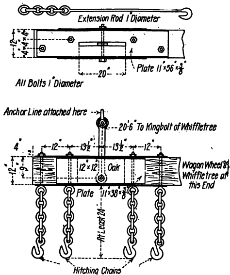
Fig. 44. Details of a Stump Puller
